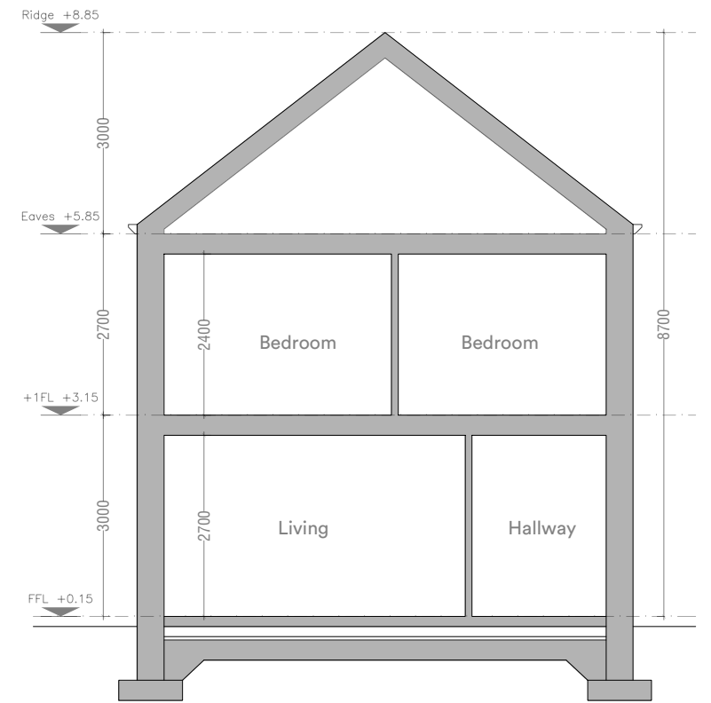
House Type M2 Detached Section A.A
