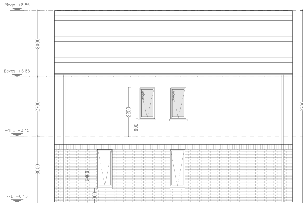
House Type M2 Detached Side Elevation
